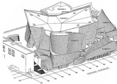
WALT DISNEY CONCERT HALL: AXONOMETRIC DRAWING, Gehry and Partners, LA Phil
